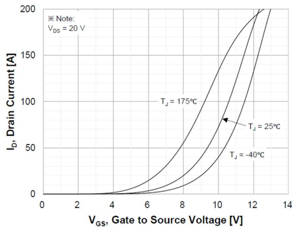
Figure 5. Transfer Characteristic
